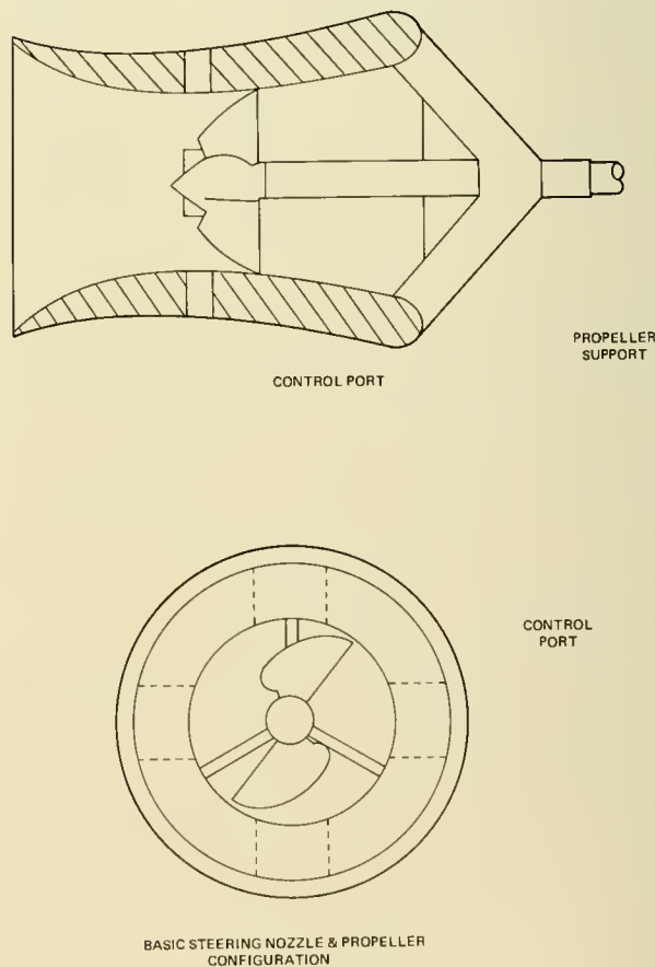
Fig. 8.20 Wake steering nozzle and propeller. [From Ref. (13)]
